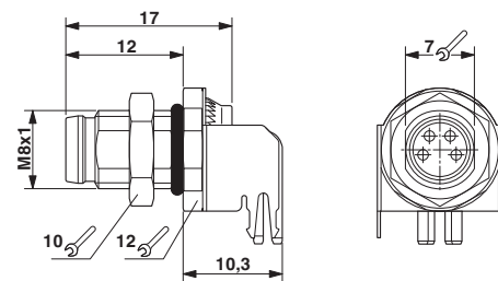
M8 flush-type plug
