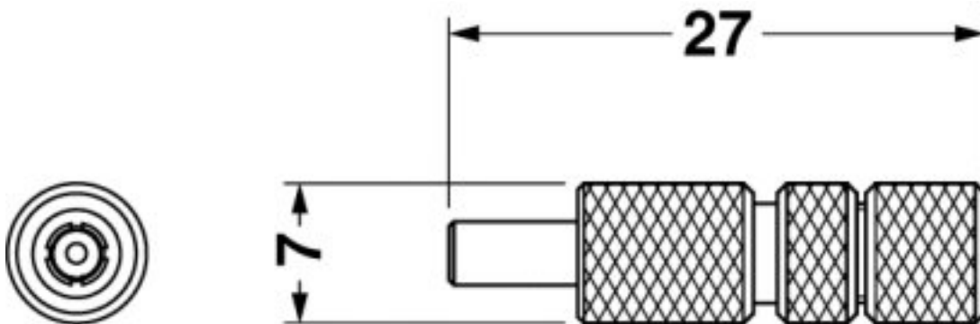
Dimensioned drawing
