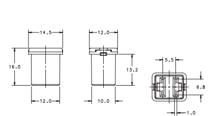
Dimensions Low Profile JCASER®
