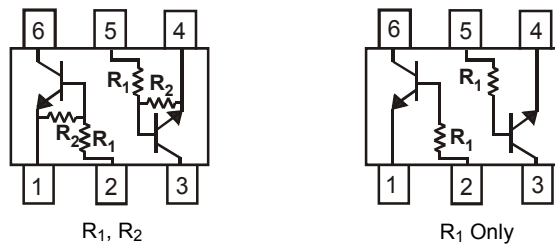
SCHMATIC DIAGRAM, TOP VIEW
