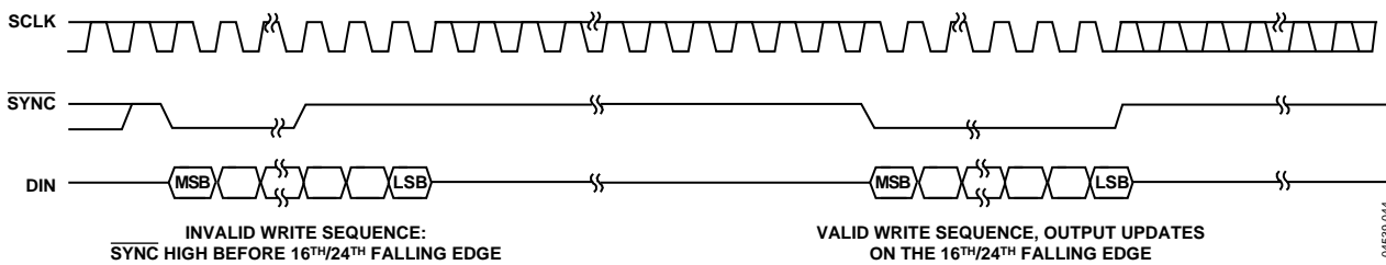
Figure 43. SYNC Interrupt Facility
