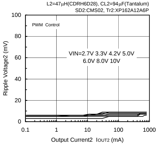
FOSC=180kHz, VOUT2=3.3V
