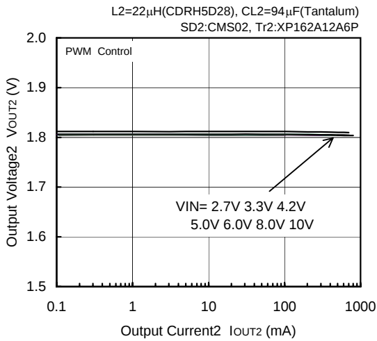
FOSC=300kHz, V OUT2 =1.8V
