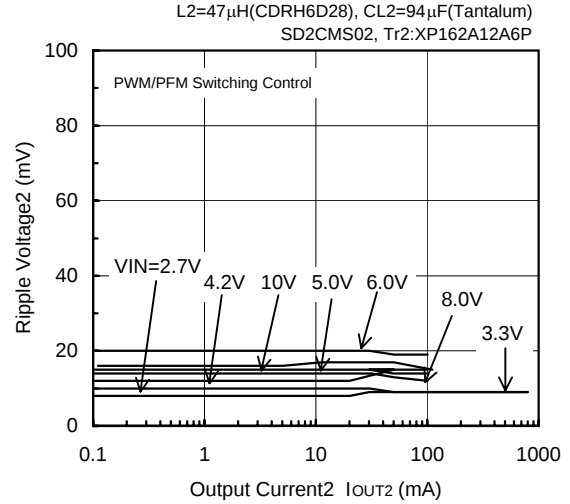
FOSC=180kHz, VOUT2=1.0V
