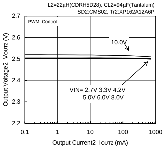
L2=22μH(CDRH5D28), CL2=94μF(Tantalum) SD2:CMS02, Tr2:XP162A12A6P
