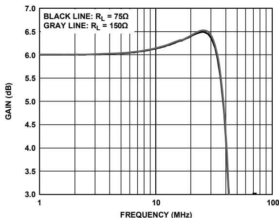
Figure 8. Flatness Response vs. Load
