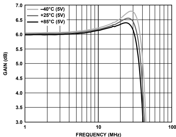
Figure 9. Flatness Response vs. Temperature
