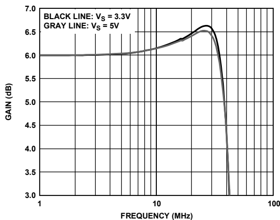
Figure 7. Flatness Response vs. Supply
