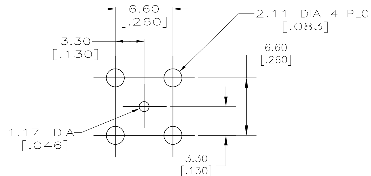
PCB CONFIGURATION
