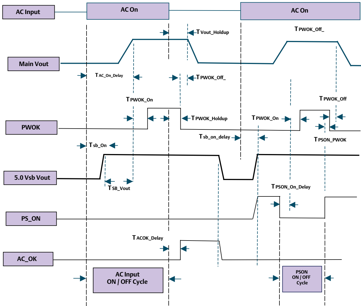
Timing Diagram
