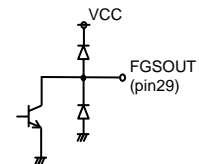
○ OFGSOUT pin
