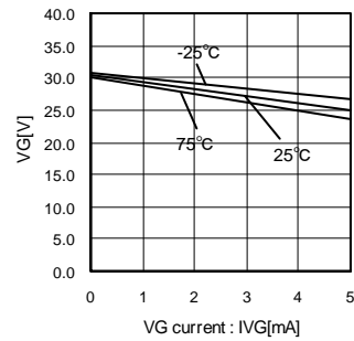
Fig.6 VG Voltage (BD6762FV)
