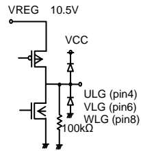
○ Low-side gate
