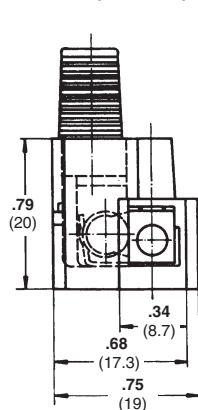
1003Si/1 (1 Circuit)
