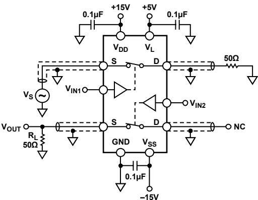
Figure 23. Channel-to-Channel Crosstalk
