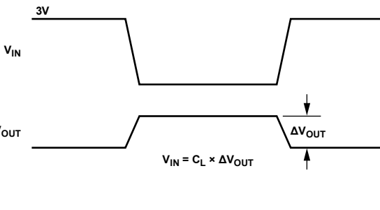
Figure 21. Charge Injection
