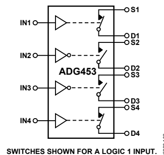
Figure 3. ADG453
