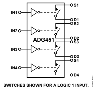
Figure 1. ADG451
