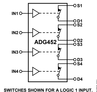
Figure 2. ADG452
