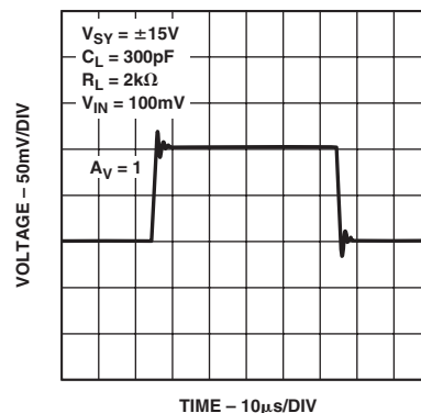
TPC 24. Small Signal Transient Response
