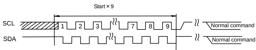
Figure 34.-(c) START×9 + command input
