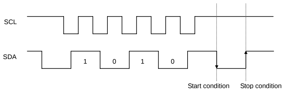
Figure 37. Case of cancel by start, stop condition during Slave Address Input
