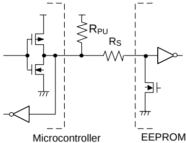
Figure 39. I/O Circuit Diagram
