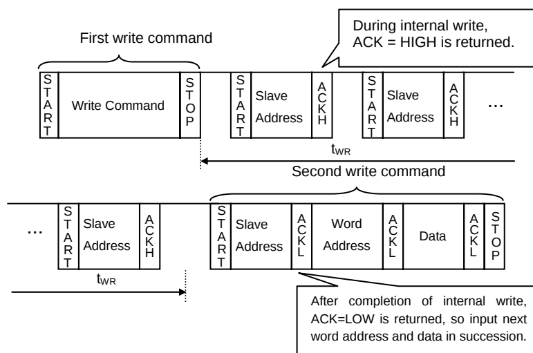
Figure 35. Case of continuous write by Acknowledge Polling
