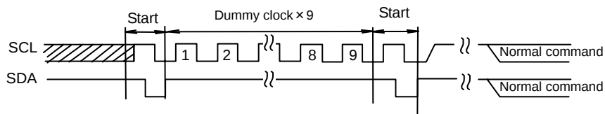
Figure 34.-(b) The case of START + dummy clock×9 + START + command input
