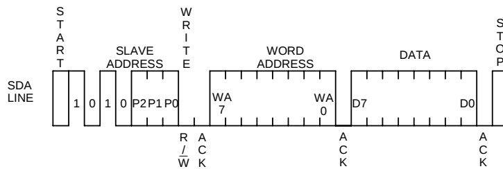
Figure 29. Byte Write Cycle
