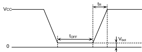
Figure 45. Rise Waveform Diagram
