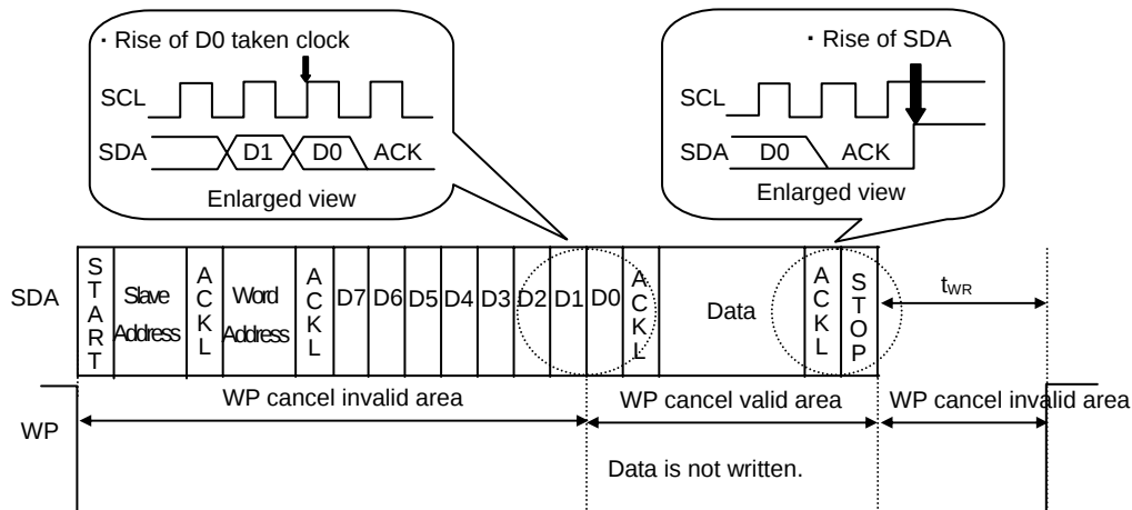
Figure 36. WP Valid Timing
