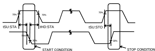
Figure 1-(b). Start-Stop Bit Timing
