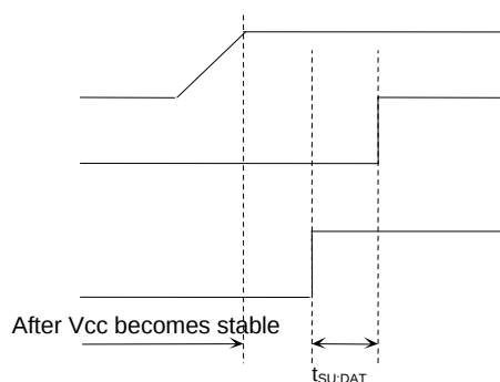
Figure 47. When SCL='L' and SDA='L'
