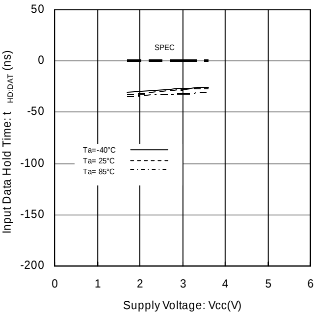
Figure 18. Input Data Hold Time vs Supply Voltage
