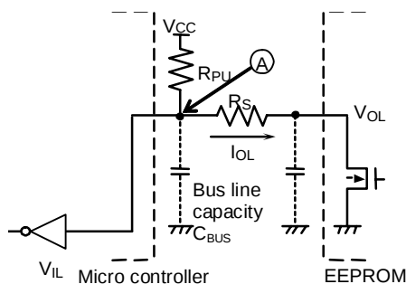
Figure 41. I/O Circuit Diagram
