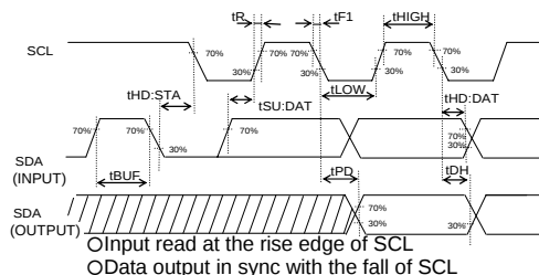
Figure 1-(a). Serial Input / Output Timing
