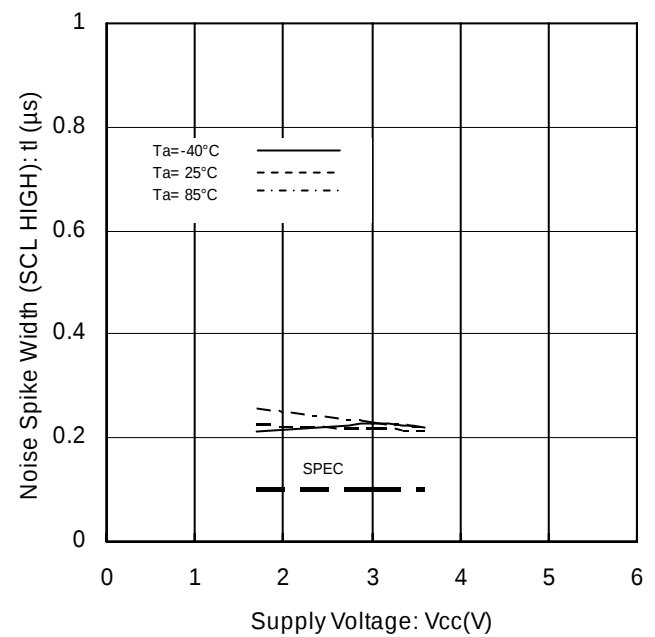
Figure 24. Noise Spike Width vs Supply Voltage (SCL H)
