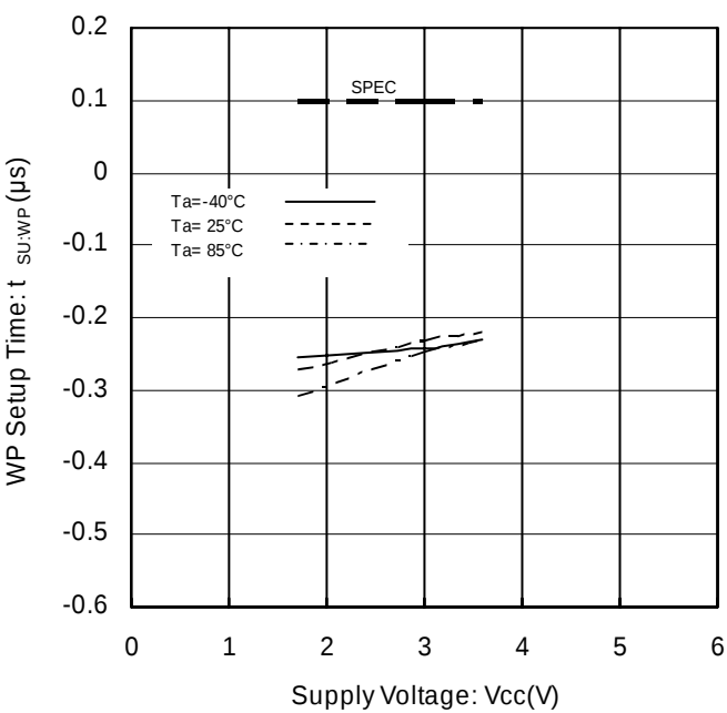
Figure 26. WP Setup Time vs Supply Voltage
