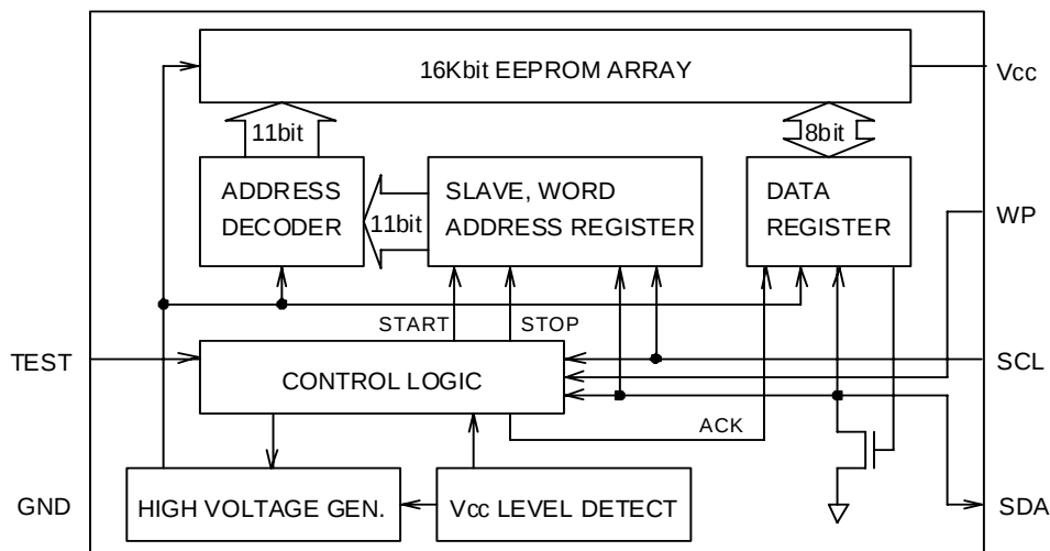
Figure 2. Block Diagram
