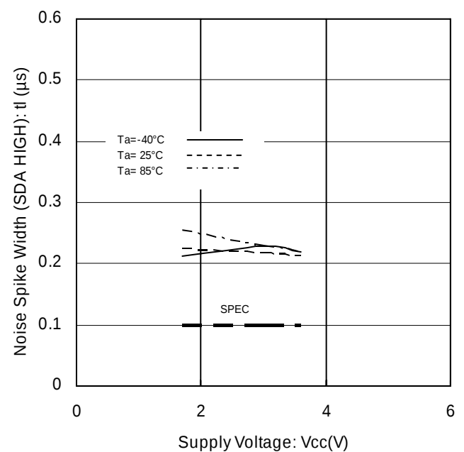
Figure 25. Noise Spike Width vs Supply Voltage (SDA H)
