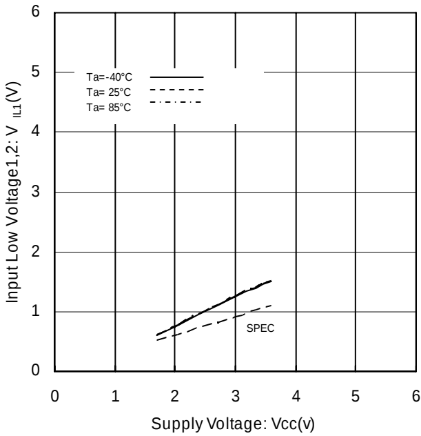
Figure 5. Input Low Voltage1 vs Supply Voltage
