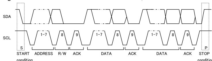
Figure 28. Data Transfer Timing
