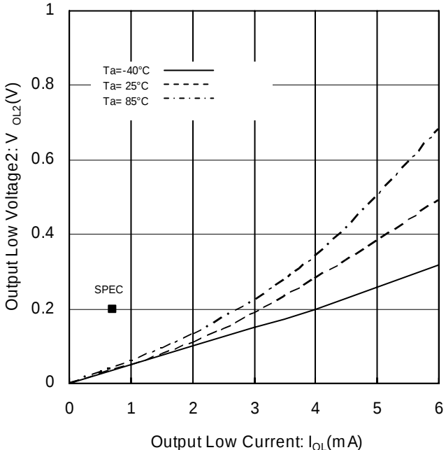
Figure 7. Output Low Voltage2 vs Output Low Current ( V_{CC} = 1.7\text{V} )
