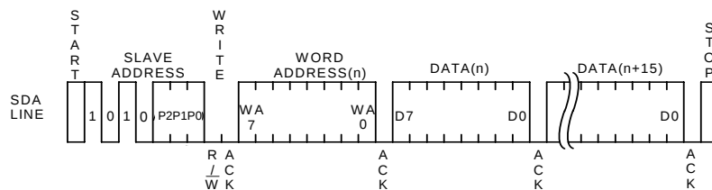
Figure 30. Page Write Cycle
