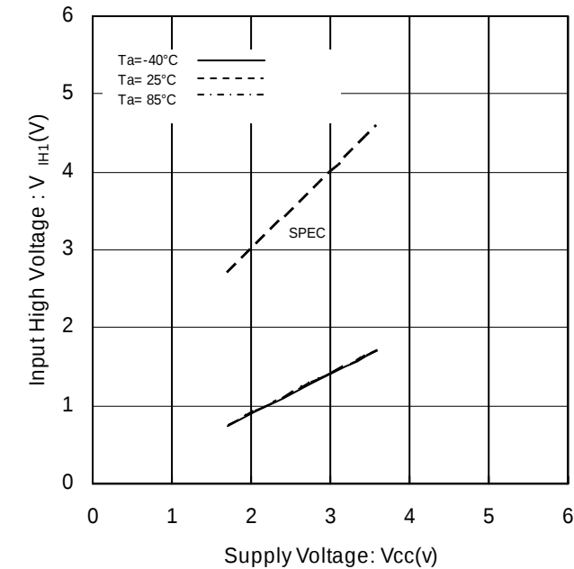
Figure 4. Input High Voltage1 vs Supply Voltage
