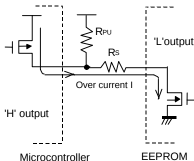
Figure 42. I/O circuit diagram
