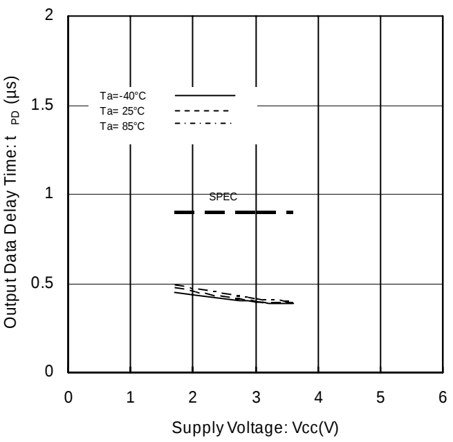
Figure 21. Output Data Delay Time vs Supply Voltage (HIGH)
