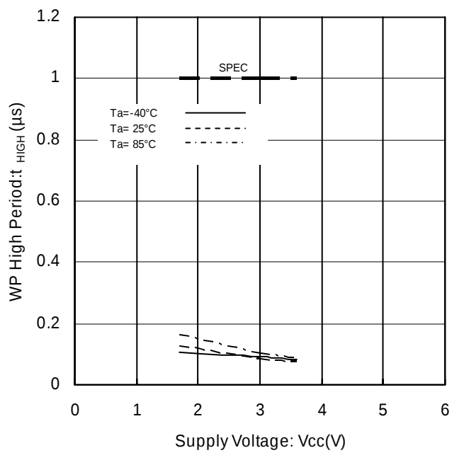
Figure 27. WP High Period vs Supply Voltage
