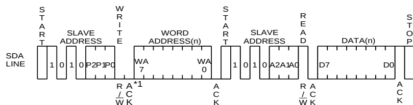
Figure 31. Random Read Cycle
