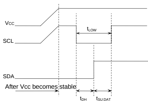
Figure 46. When SCL='H' and SDA='L'
