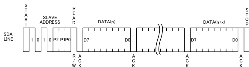
Figure 33. Sequential Read Cycle (in the case of Current Read Cycle)
