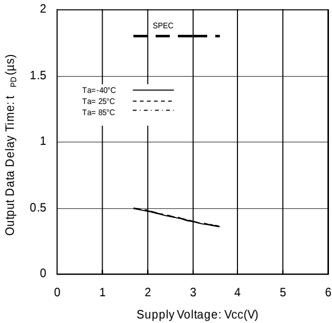
Figure 20. Output Data Delay Time vs Supply Voltage (LOW)
