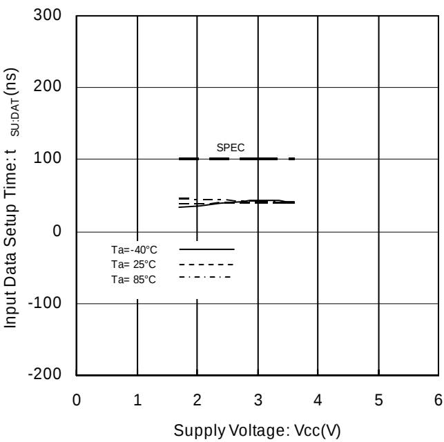
Figure 19. Input Data Setup Time vs Supply Voltage
