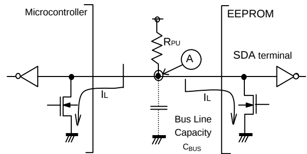
Figure 38. I/O Circuit Diagram
