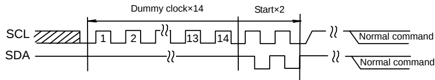
Figure 34.-(a) The case of dummy clock×14 + START+START+ command input
