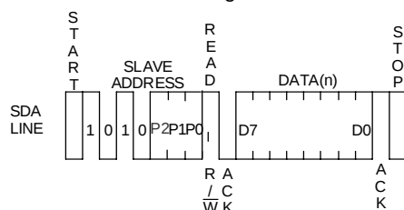
Figure 32. Current Read Cycle
