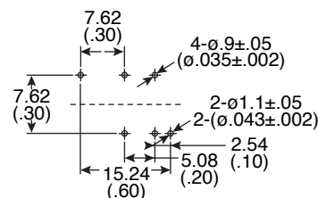
P.C. Mounting
