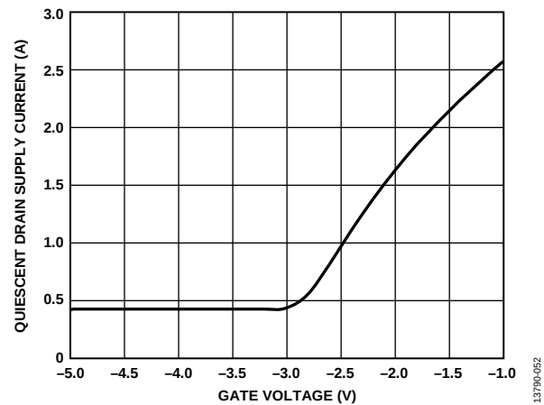
Figure 50. Quiescent Drain Supply Current vs. Gate Voltage
