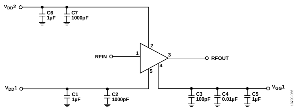
Figure 57. Typical Application Circuit
