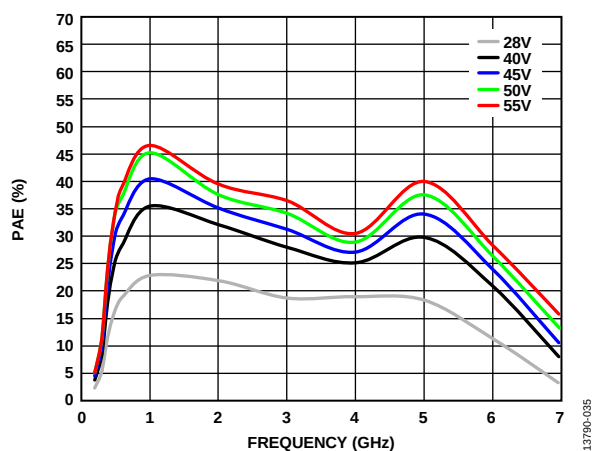
Figure 34. PAE vs. Frequency at Various Voltages, Input Power = 24 dBm
