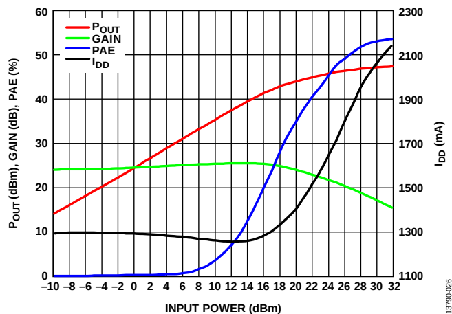
Figure 42. P_{OUT} , Gain, PAE, and Total Supply Current with RF Power Applied ( I_{DD} ) vs. Input Power, Frequency = 1 GHz
