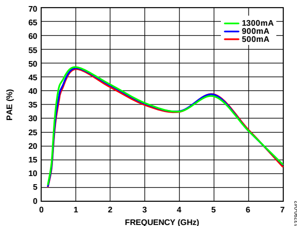
Figure 38. PAE vs. Frequency at Various Quiescent Currents ( I_{DD1} + I_{DD2} ), Input Power = 28 dBm
