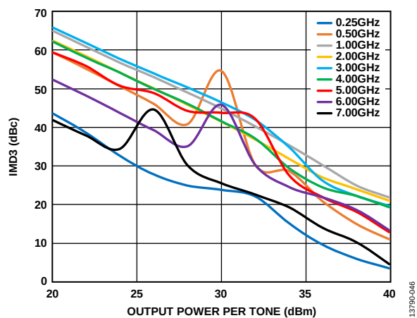
Figure 46. Upper Third-Order Intermodulation Distortion (IMD3) vs. Output Power per Tone at Various Frequencies
