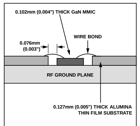
Figure 55. Die Without the Moly Tab
