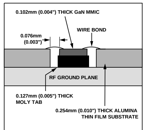
Figure 56. Die With the Moly Tab
