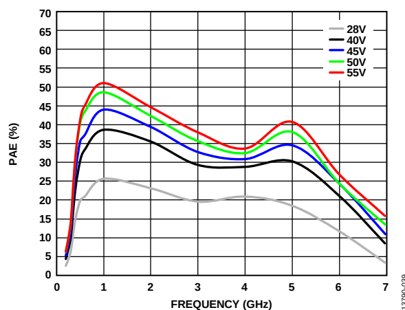
Figure 37. PAE vs. Frequency at Various Voltages, Input Power = 28 dBm
