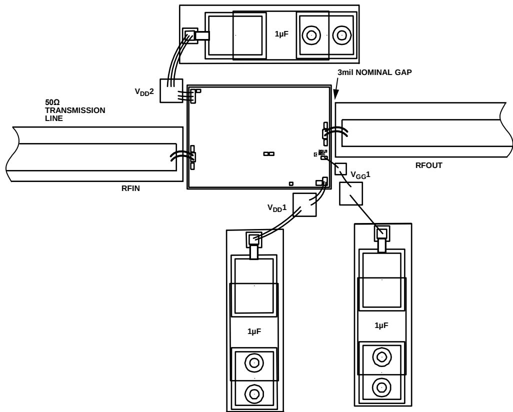
Figure 58. Assembly Diagram
