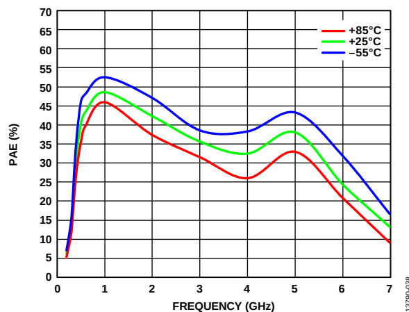
Figure 36. PAE vs. Frequency at Various Temperatures, Input Power = 28 dBm
