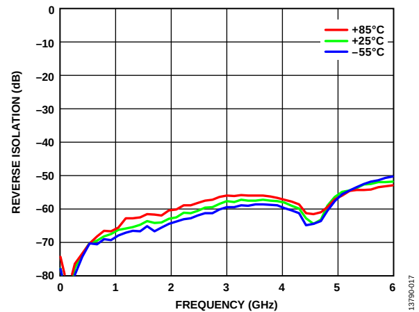
Figure 18. Reverse Isolation vs. Frequency at Various Temperatures
