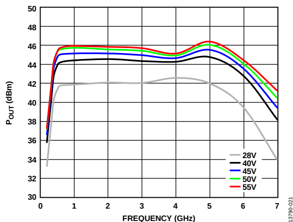
Figure 22. P_{OUT} vs. Frequency at Various Voltages, P_{IN} = 24 dBm
