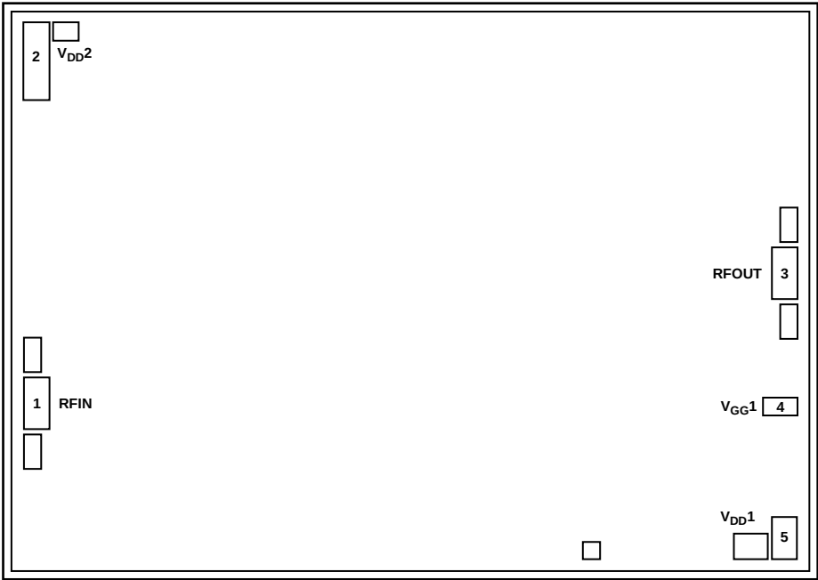
Figure 2. Pad Configuration
