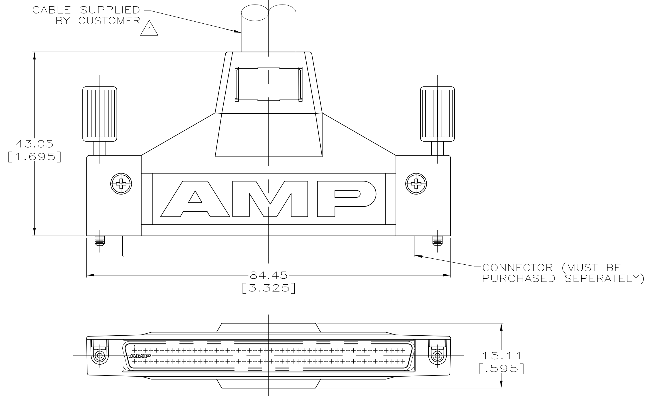
ASSEMBLED VIEW
