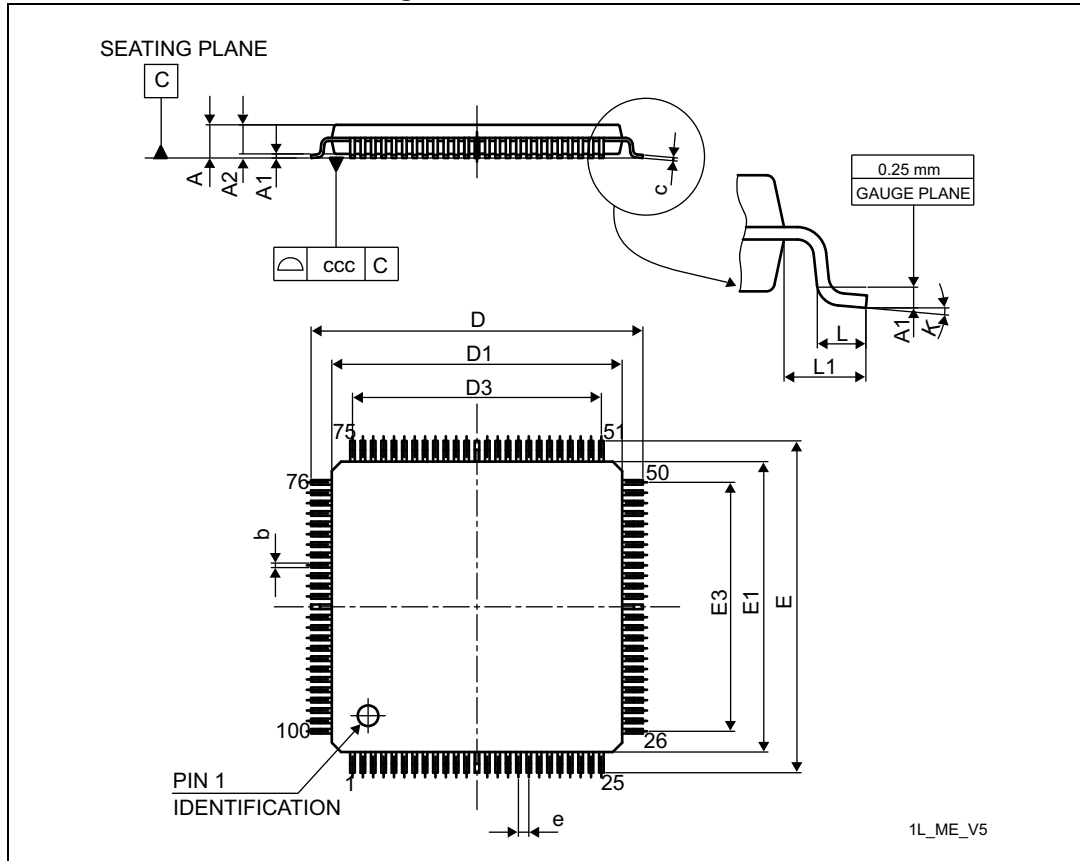
Figure 82. LQFP100 outline
