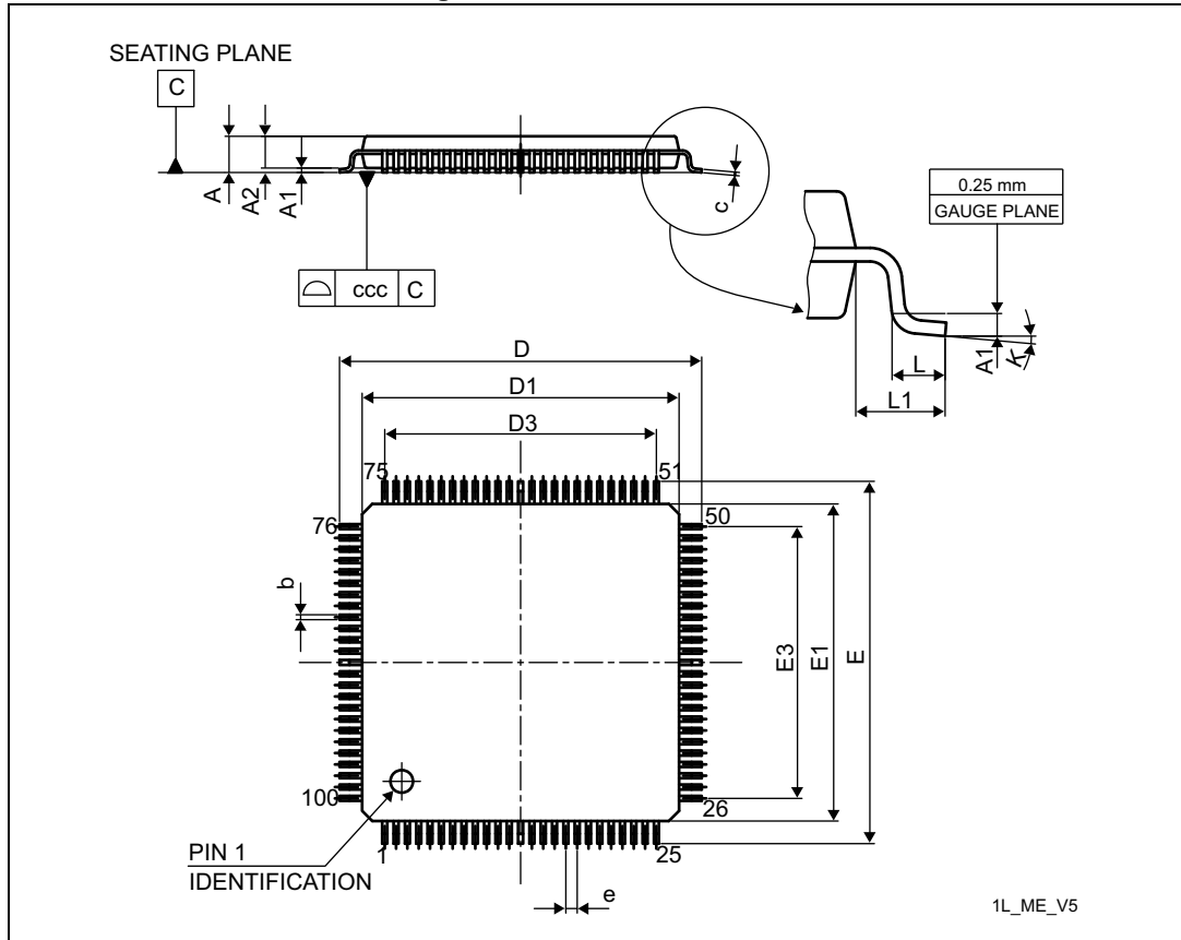
Figure 82. LQFP100 outline
