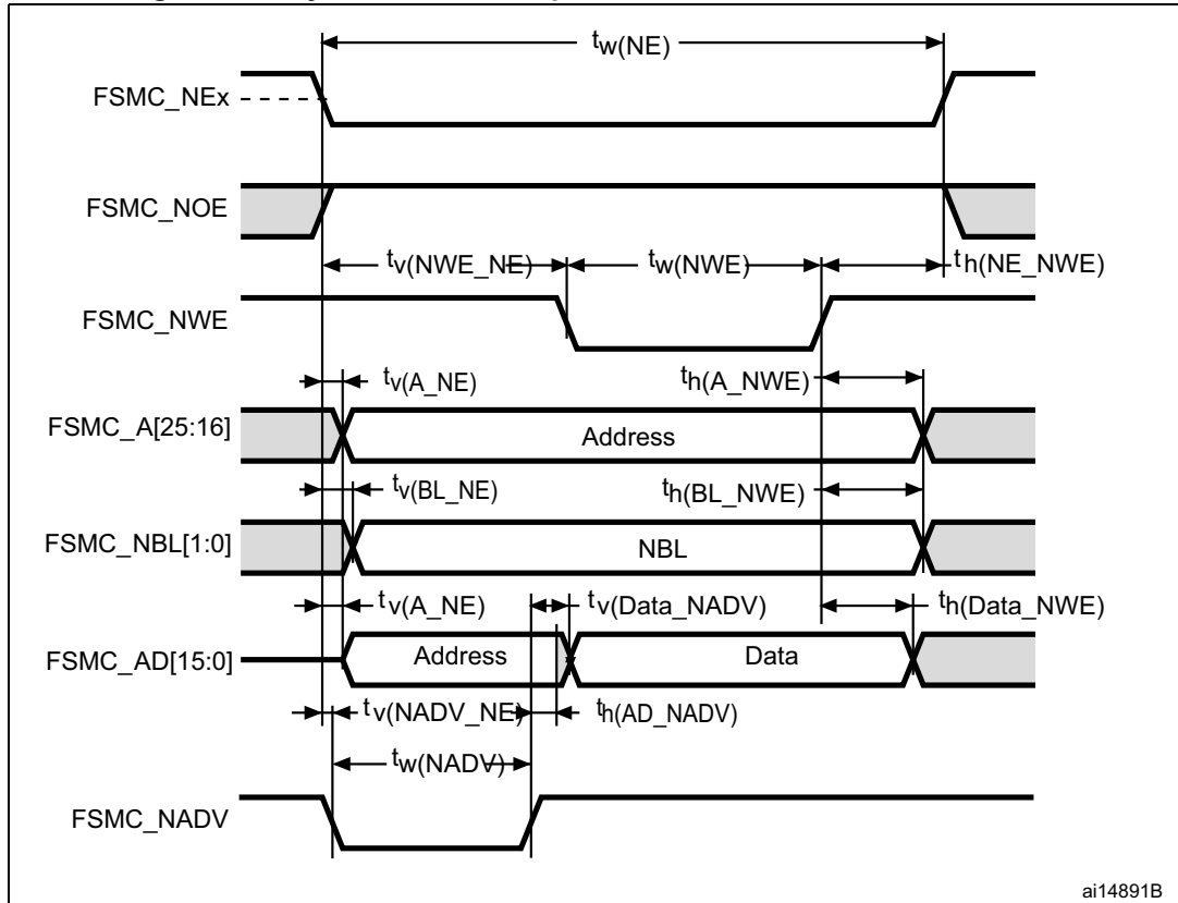
Figure 60. Asynchronous multiplexed PSRAM/NOR write waveforms
