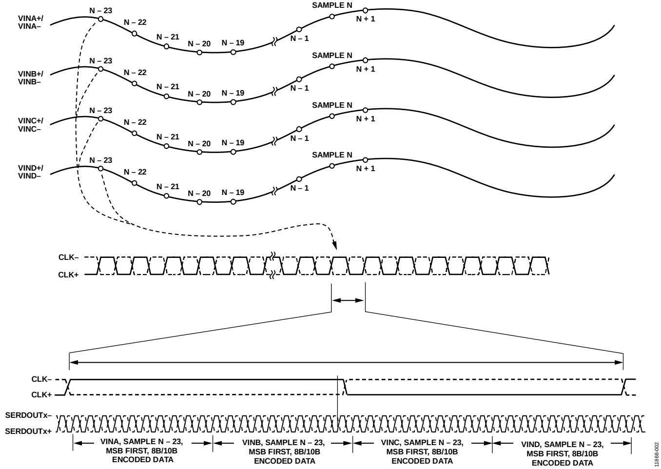
Figure 2. Data Output Timing, M = 4 , L = 1
