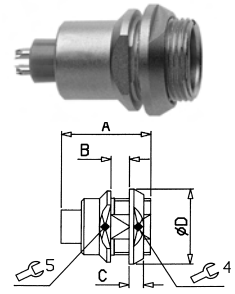
EP : Fixed receptacle, back panel mounting
