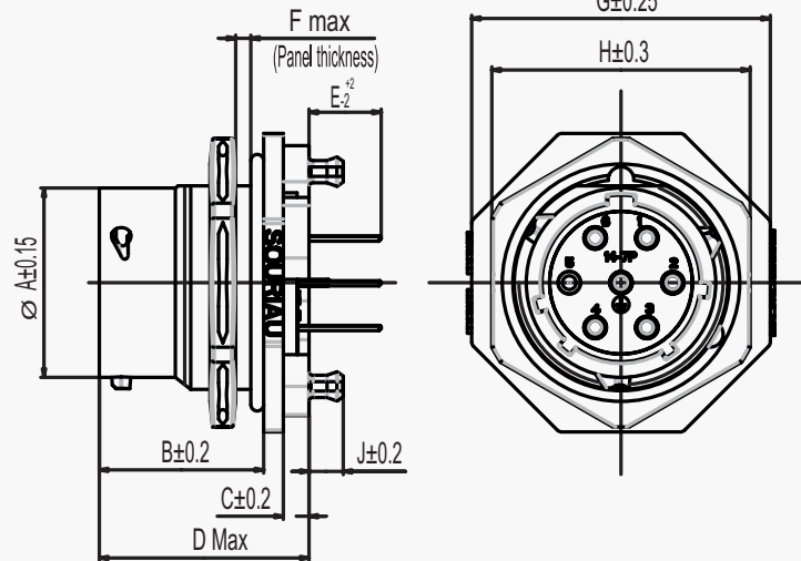
MATING FACE
