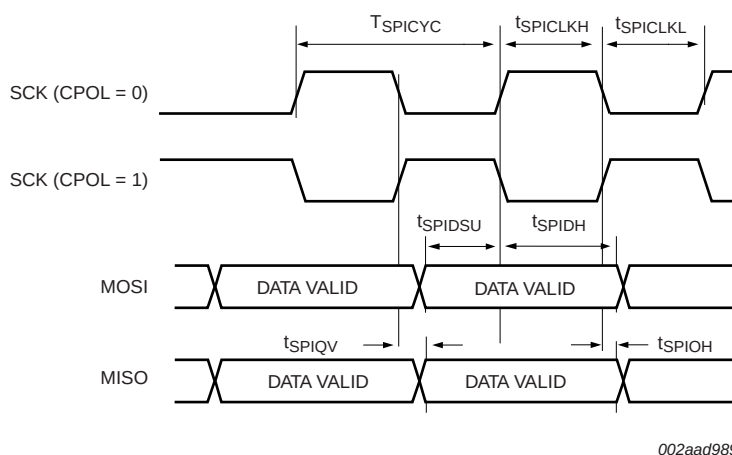
Fig 22. SPI slave timing (CPHA = 0)
