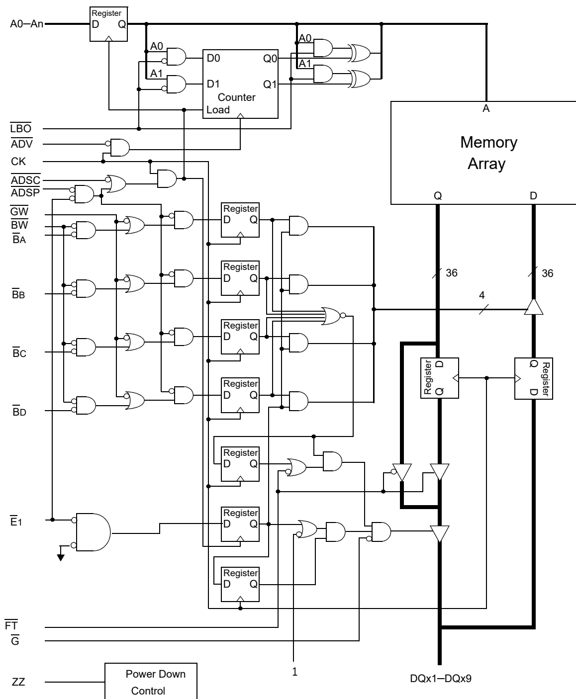
GS8256418/36 Block Diagram
