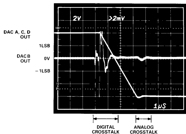
Figure 7. Output Crosstalk
