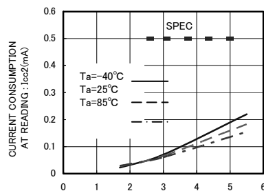
Fig.12 Current consumption at READ operation I_{CC2} (fsc1=400kHz BR24T01/02/04/08/16/32/64/128/256-W)
