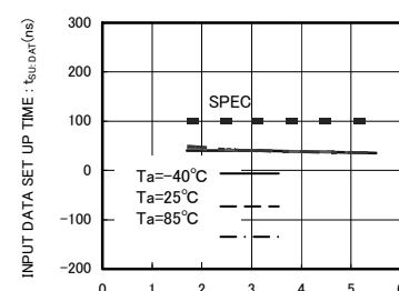
Fig.23 Input Data Setup Time t_{SU:DAT(HIGH)}
