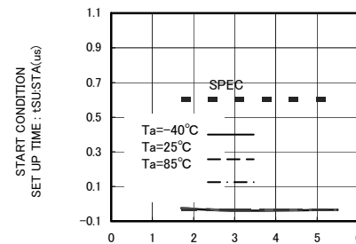
Fig.20 Start Condition Setup Time t_{SU:STA}
