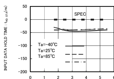
Fig.21 Input Data Hold Time t_{HD:DAT(HIGH)}
