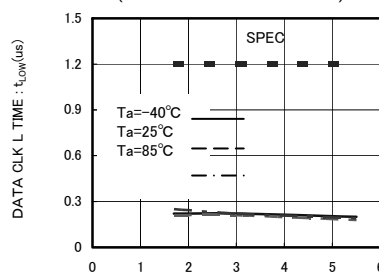
Fig.18 Data clock Low Period t_{LOW}
