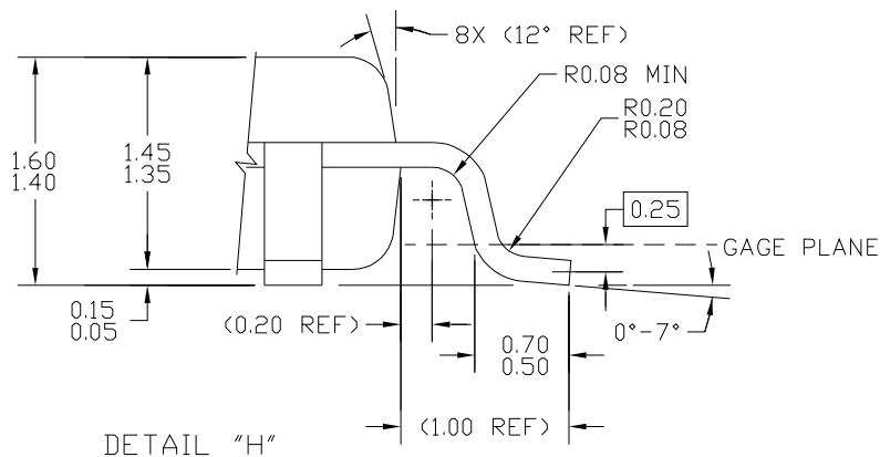
DETAIL "H"
