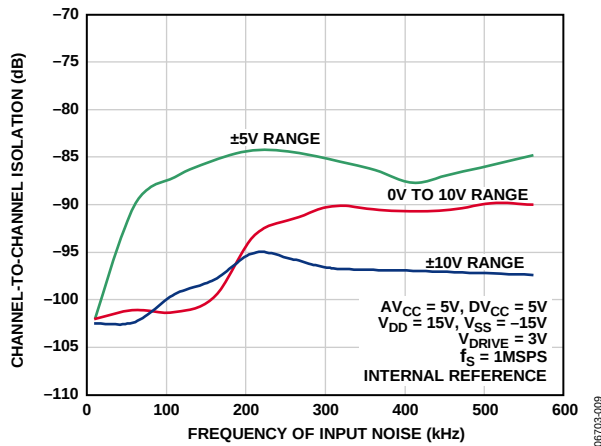
Figure 9. Channel-to-Channel Isolation
