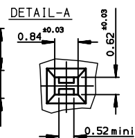
DETAIL OF PRESS-IN PEGS
