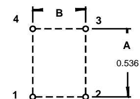
PIN MOUNTING
