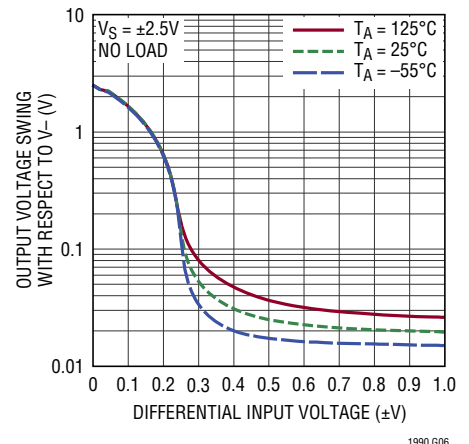
Output Voltage Swing vs Input Voltage (Low)
