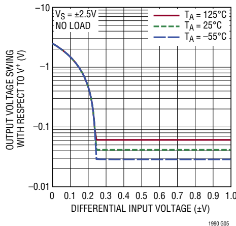
Output Voltage Swing vs Input Voltage (High)
