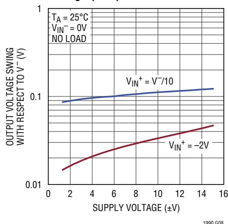
Output Voltage Swing vs Supply Voltage (Low)
