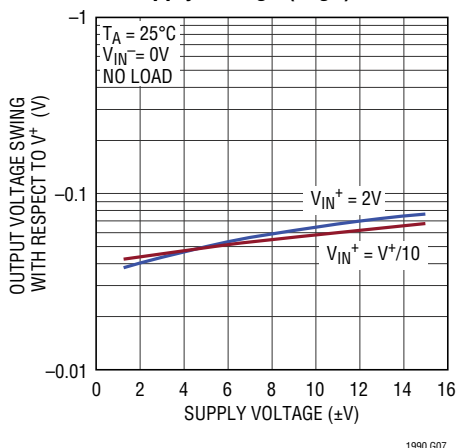
Output Voltage Swing vs Supply Voltage (High)
