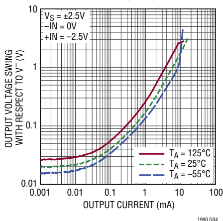
Output Voltage Swing vs Load Current (Sink)
