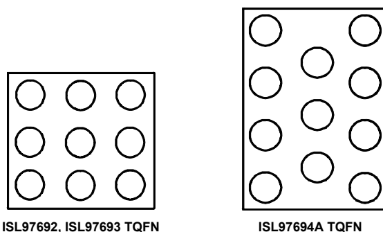
FIGURE 32. VIA PATTERN
