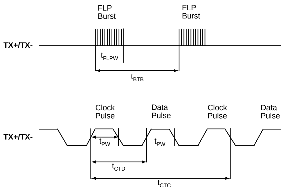
Figure 13. Auto-Negotiation Timing
