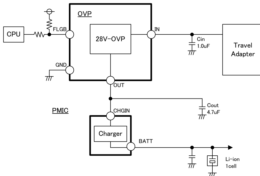
Fig. 4 Application Circuit
