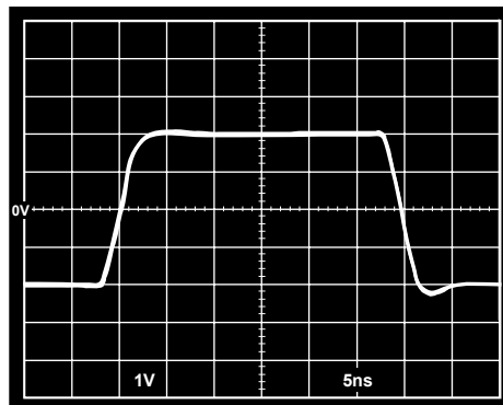
Figure 9. Large Step Response, G = -1 (See Figure 35)
