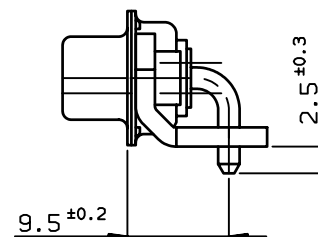
VIEW WITH POWERS CONTACTS
