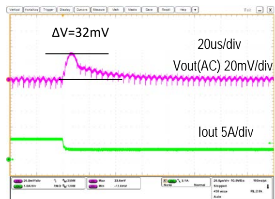
Step Load Transient Response (Vin=5.0V, Vout=1.0V, Cload=400uF, Iout=6A to 3A, 2.5A/us)
