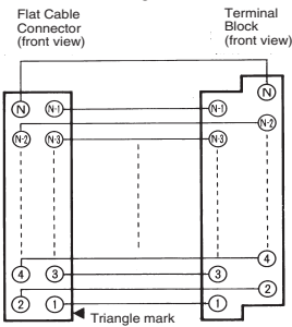
Connection Diagram
