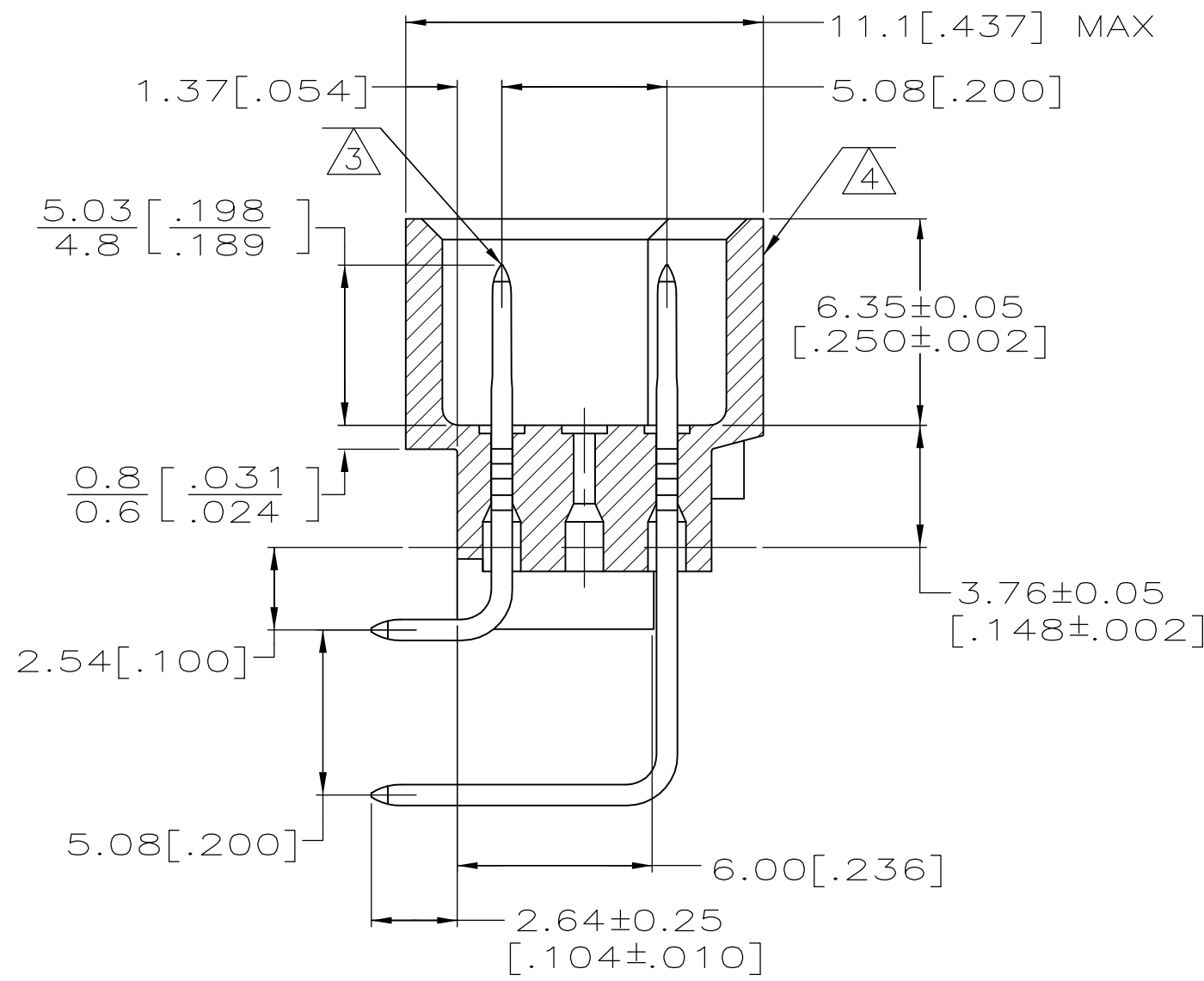
SECTION Z-Z
