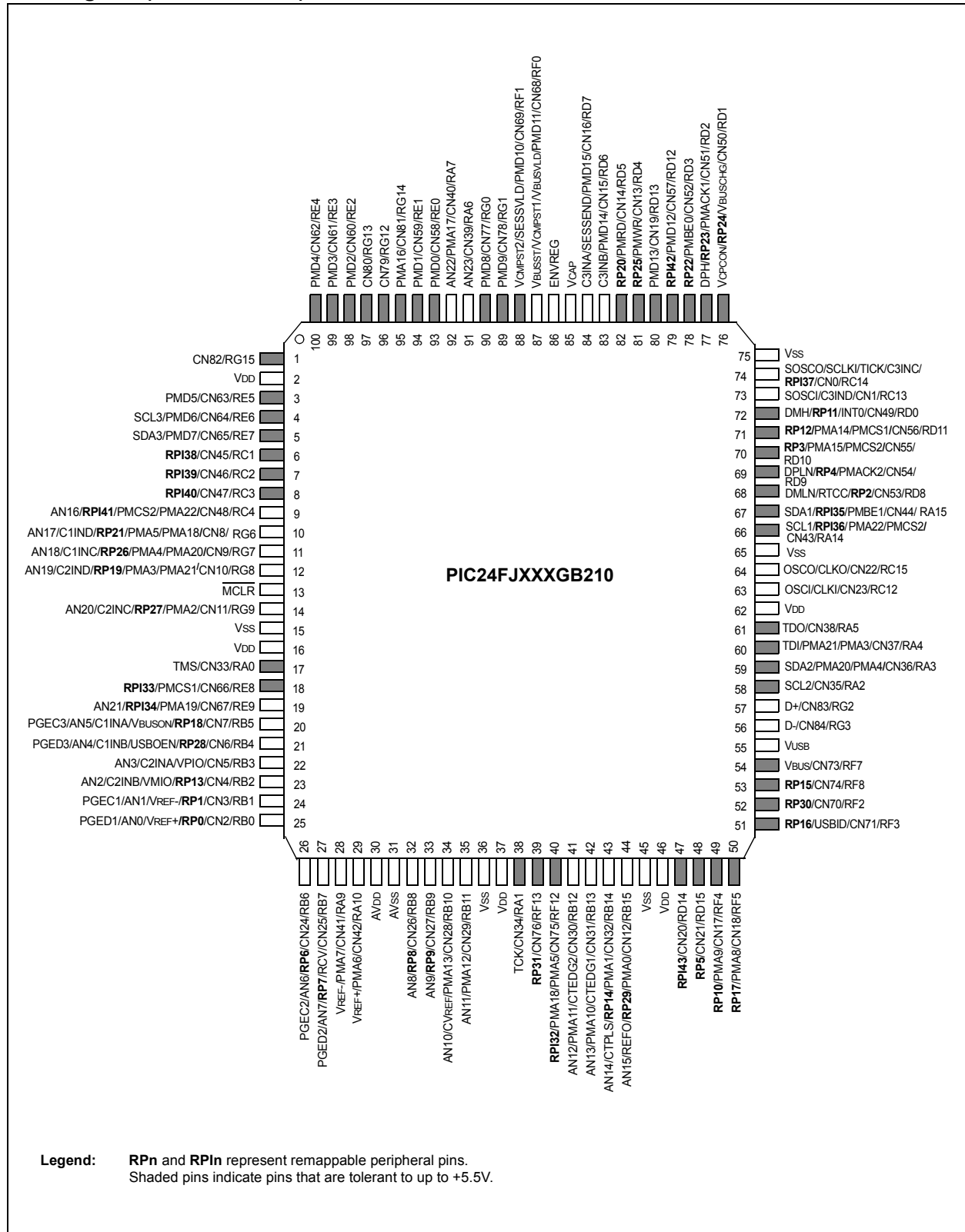
Pin Diagram (100-Pin TQFP)
