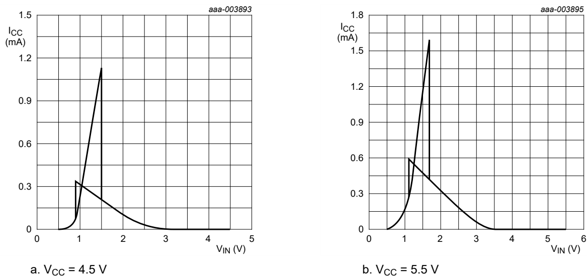
Fig. 11. Typical 74HCT132-Q100 transfer characteristics
