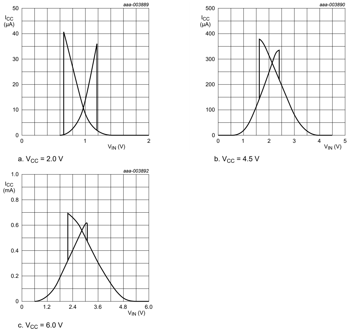
Fig. 10. Typical 74HC132-Q100 transfer characteristics
