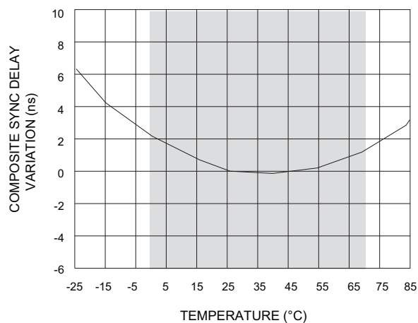
Figure 3-1: Composite Sync Delay Variation vs Temperature
