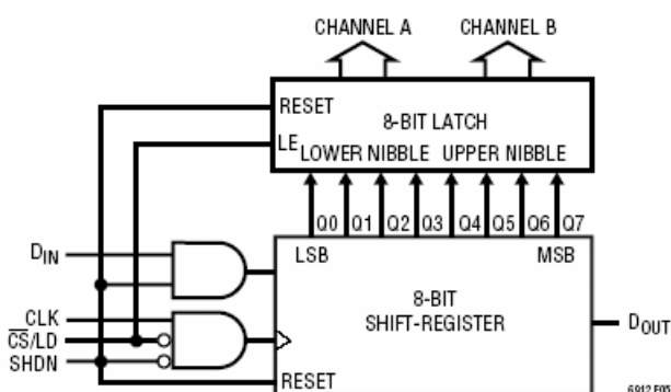
Figure 3. Block Diagram, LTC6912-1/2 Serial Interface
