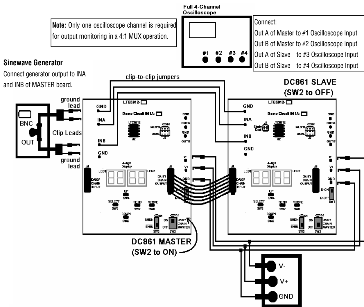
Figure 7. Quad PGA or 4:1 MUX Daisy Chain Quick Set-Up (Dual Supply Operation)
