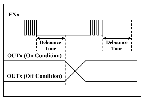
Figure 22 EN Debounced
