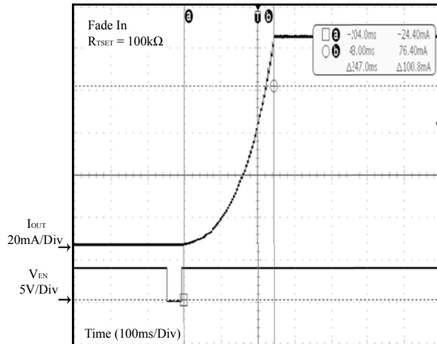
Figure 14 V_{EN} vs. I_{OUT}
