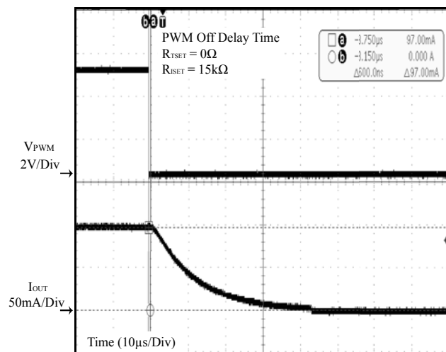
Figure 11 PWM Off Delay Time (For IS32LT3175P Only)
