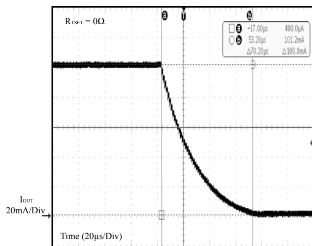
Figure 13 Instant Off
