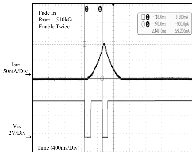
Figure 18 V_{EN} vs. I_{OUT}
