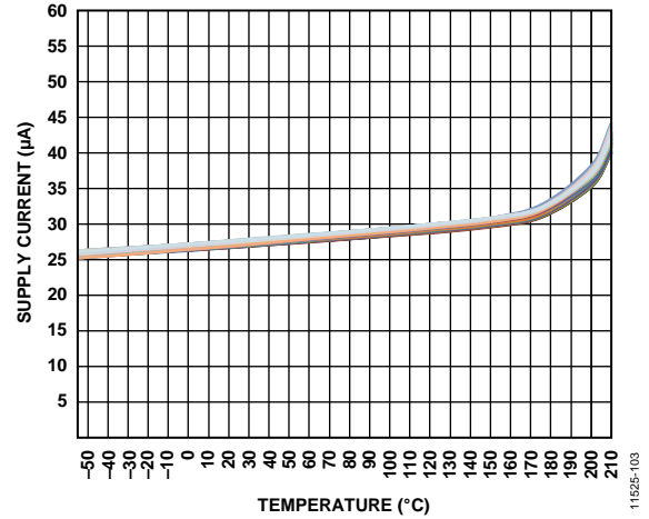
Figure 12. Supply Current ( I_{SV} ) vs. Temperature, FLATPACK Package
