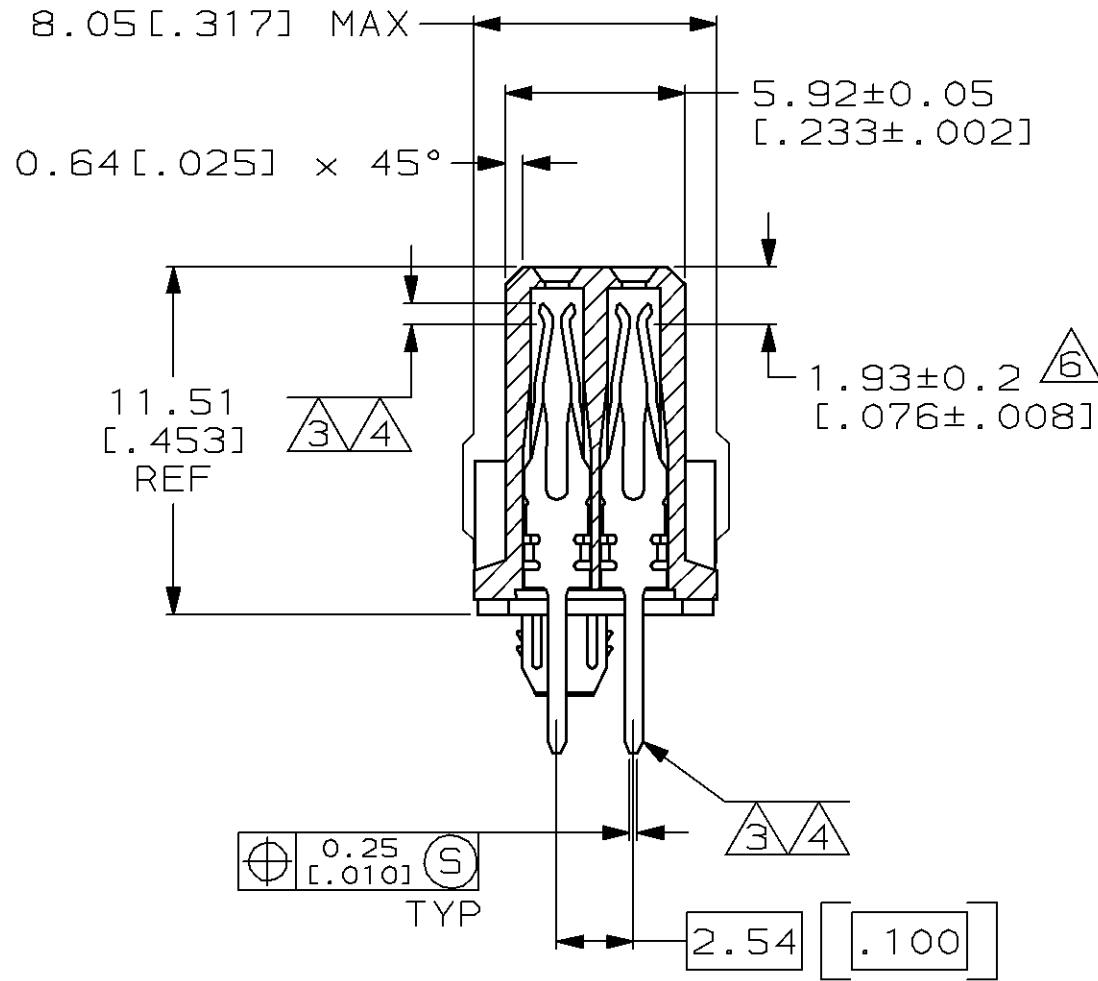
SECTION X-X
