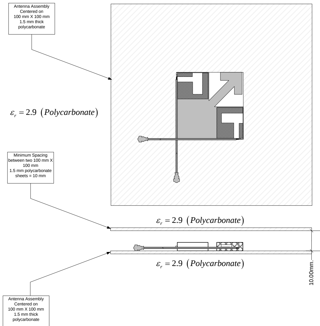
Figure 5: Minimum clearance of dielectric sheet loading on top of the antenna array
