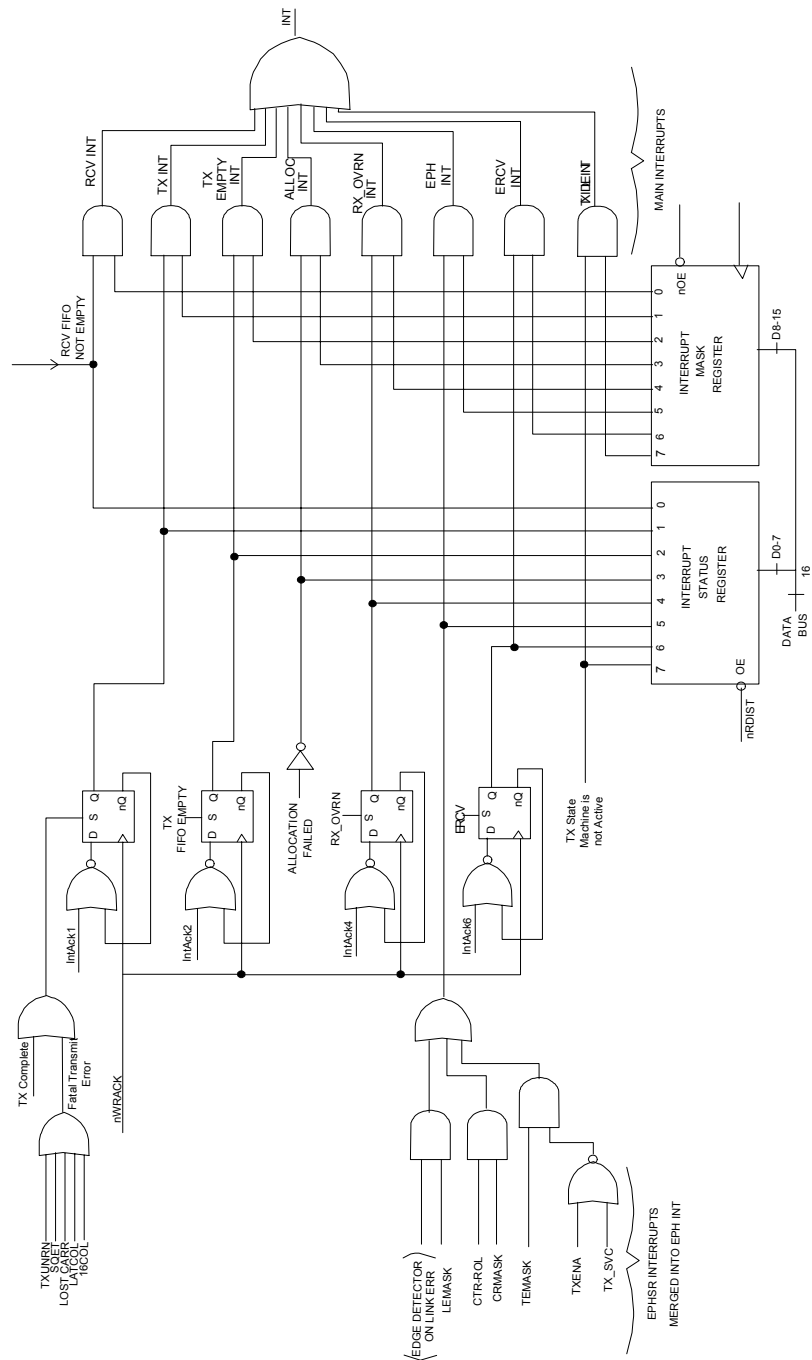
Figure 7.2 – Interrupt Structure
