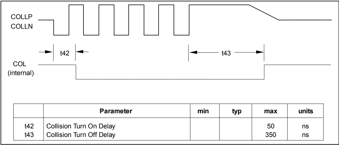
Figure 12.18 – Collision Timing (AUI)
