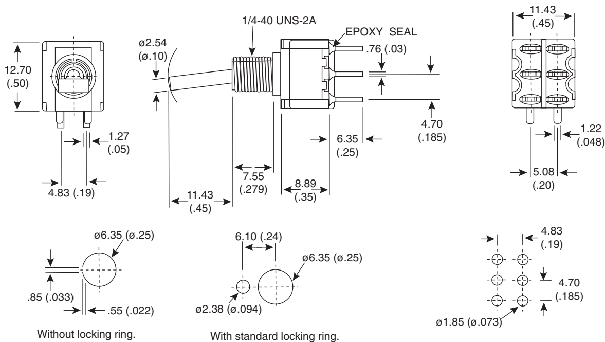
P.C. MOUNTING
